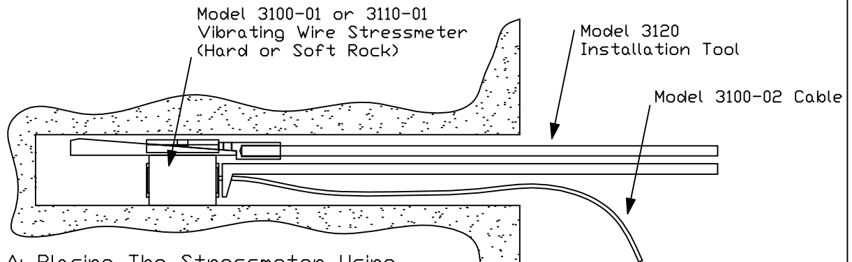
A: Placing The Stressmeter Using The Installation Tool
